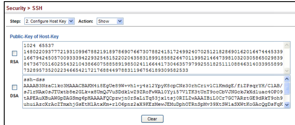
Figure 190: Showing the SSH Host Key Pair
