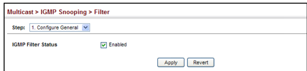
Figure 350: Enabling IGMP Filtering and Throttling
