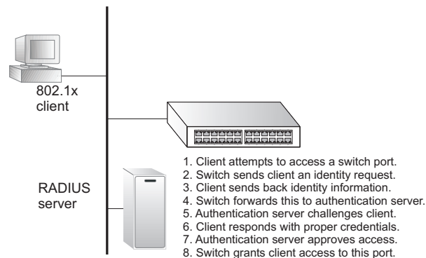
Figure 218: Configuring Port Security
