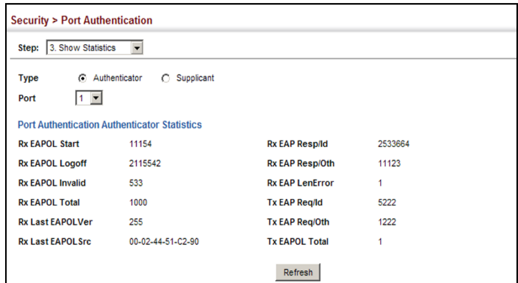
Figure 222: Showing Statistics for 802.1X Port Authenticator
