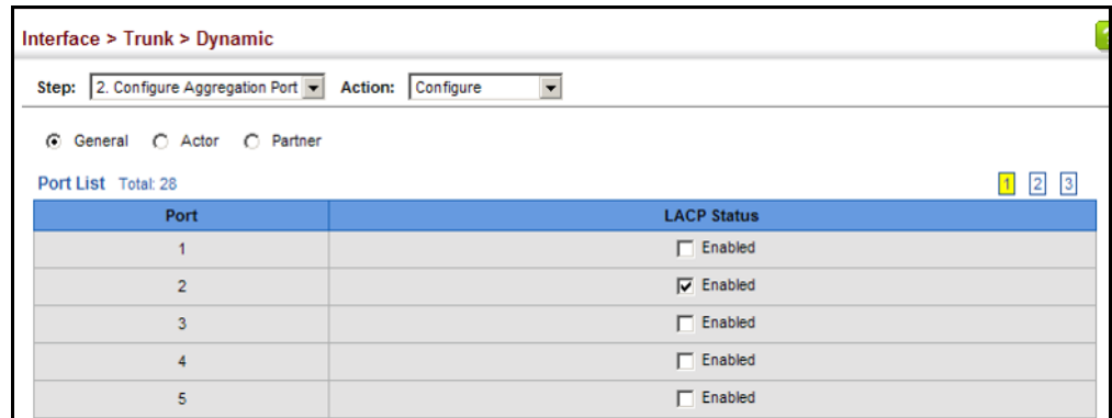
Figure 54: Enabling LACP on a Port
