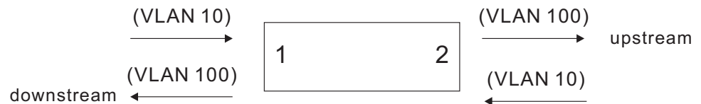
Figure 96: Configuring VLAN Translation
