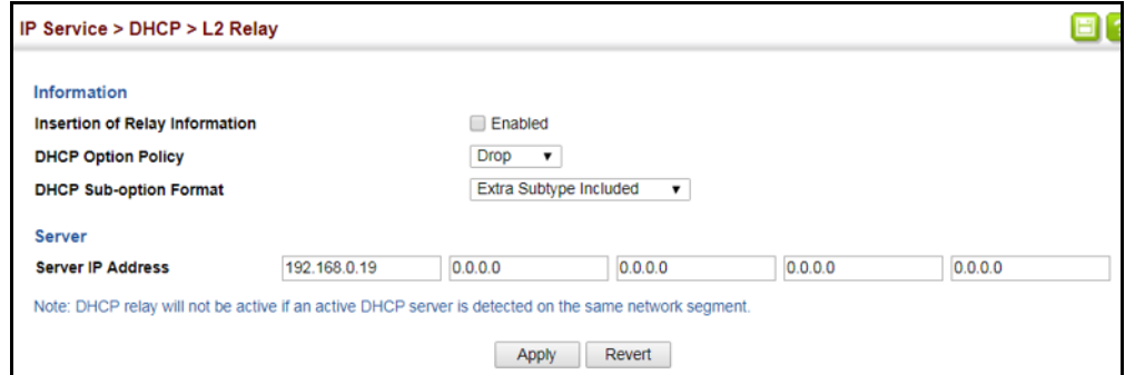
Figure 460: Configuring DHCP Relay Information Option 82 Service
