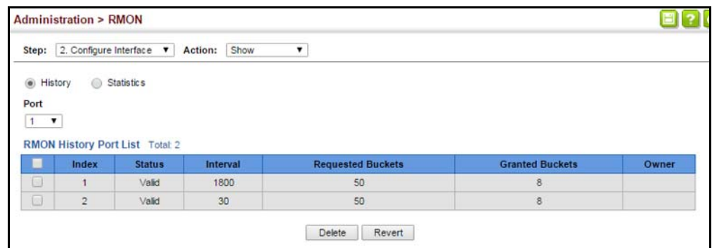
Figure 295: Showing Configured RMON History Samples
