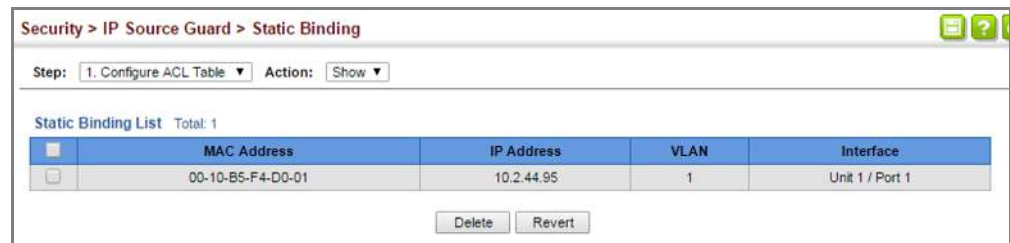
Figure 216: Displaying Static Bindings for IPv4 Source Guard
