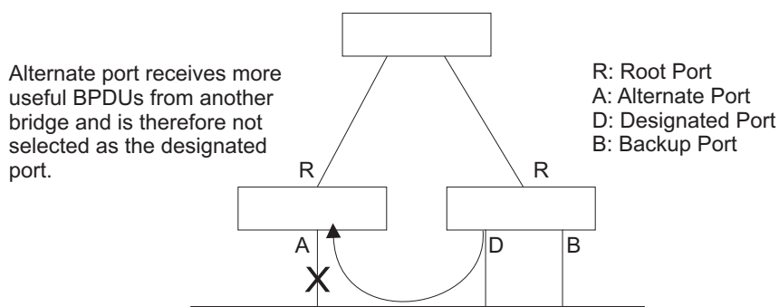
Figure 118: STA Port Roles
