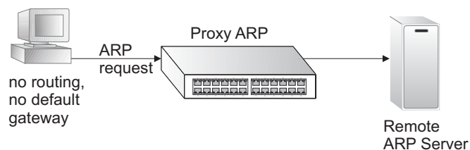
Figure 427: Proxy ARP
