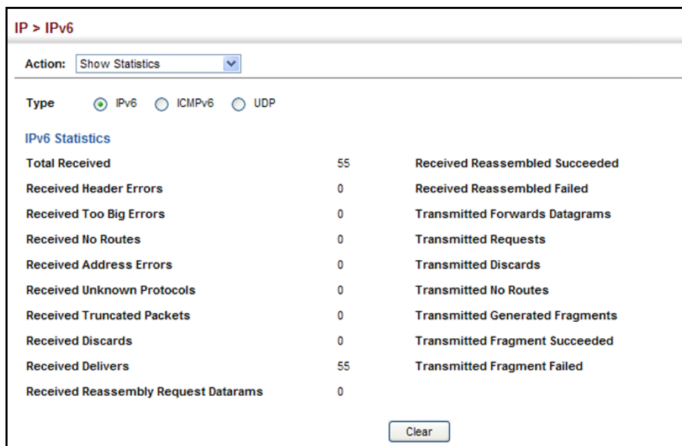
Figure 442: Showing IPv6 Statistics (IPv6)
