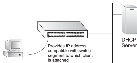
Figure 459: Layer 3 DHCP Relay Service
