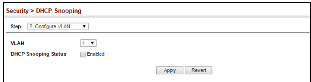
Figure 226: Configuring DHCP Snooping on a VLAN
