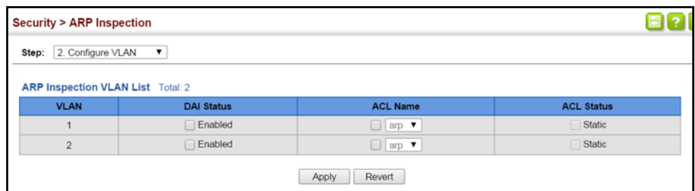
Figure 244: Configuring VLAN Settings for ARP Inspection
