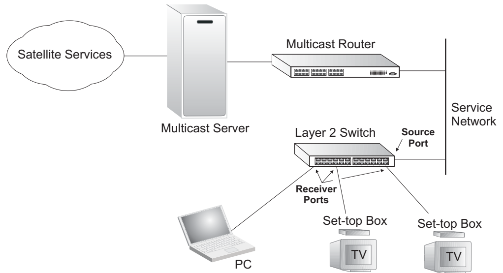
Figure 398: MVR Concept
