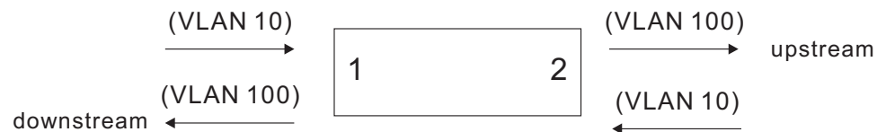
Figure 105: Configuring VLAN Translation
