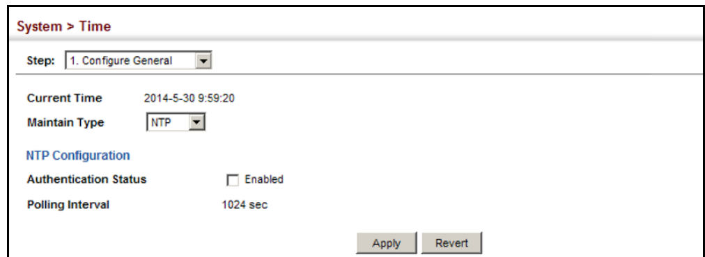
Figure 15: Configuring NTP
