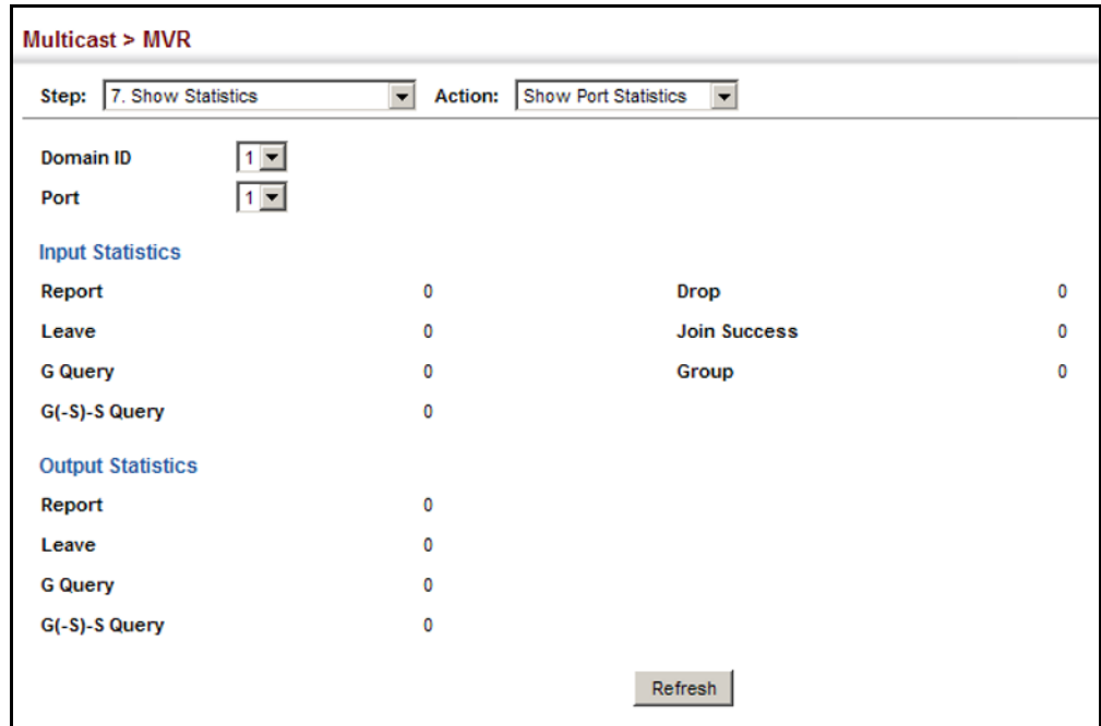
Figure 411: Displaying MVR Statistics – Port
