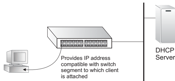
Figure 461: Layer 2 DHCP Relay Service
