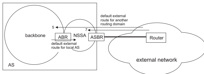
Figure 492: OSPF NSSA
